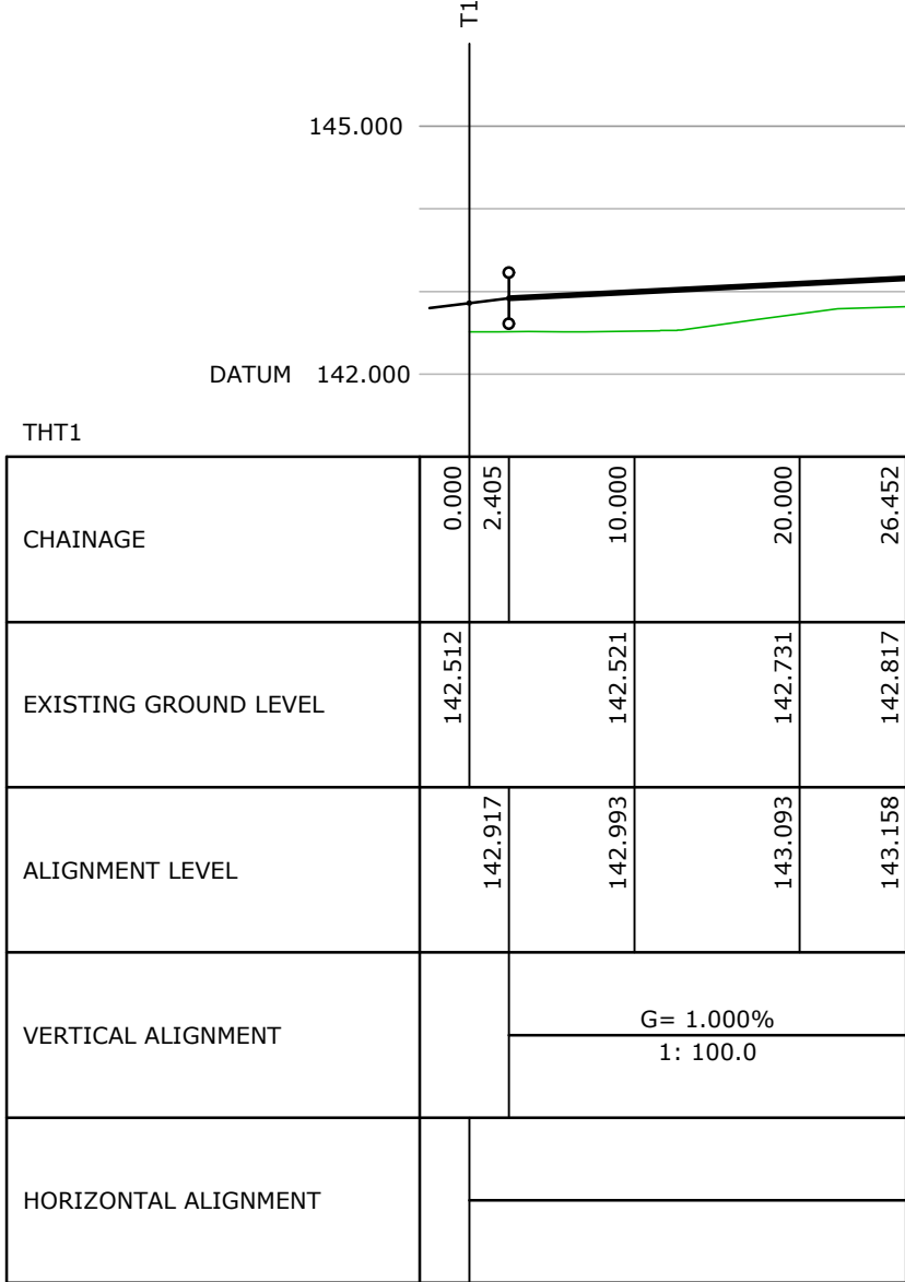
Longitudinal Section Along Turning Head Tertiary Road 1
