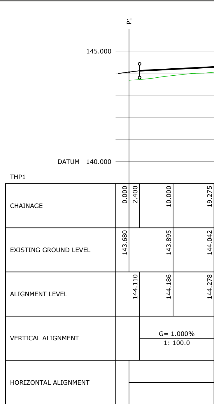
Longitudinal Section Along Turning Head Primary Road 1
