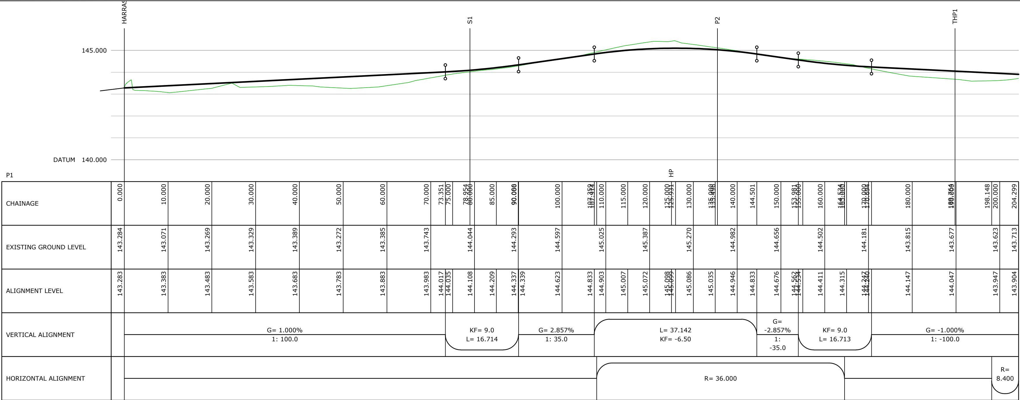
Longitudinal Section Along Primary Road 1
