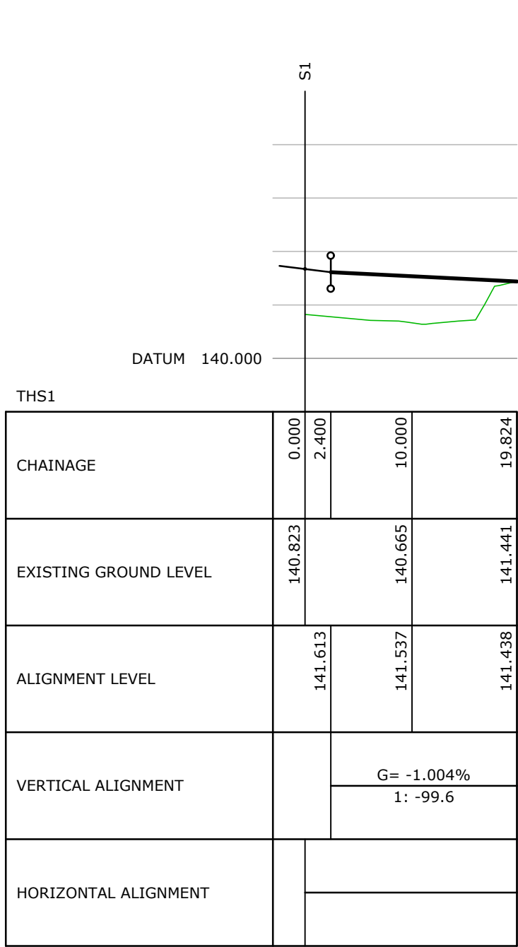
Longitudinal Section Along Turning Head Secondary Road 1
