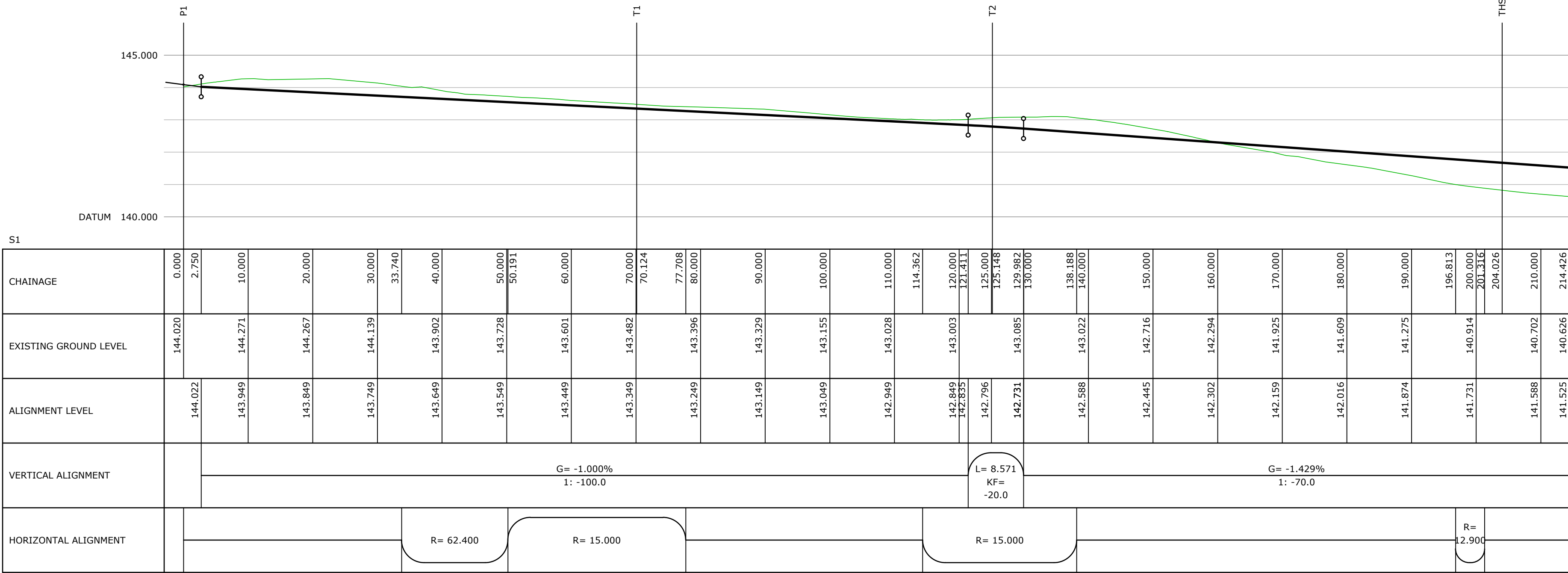
Longitudinal Section Along Secondary Road 1
