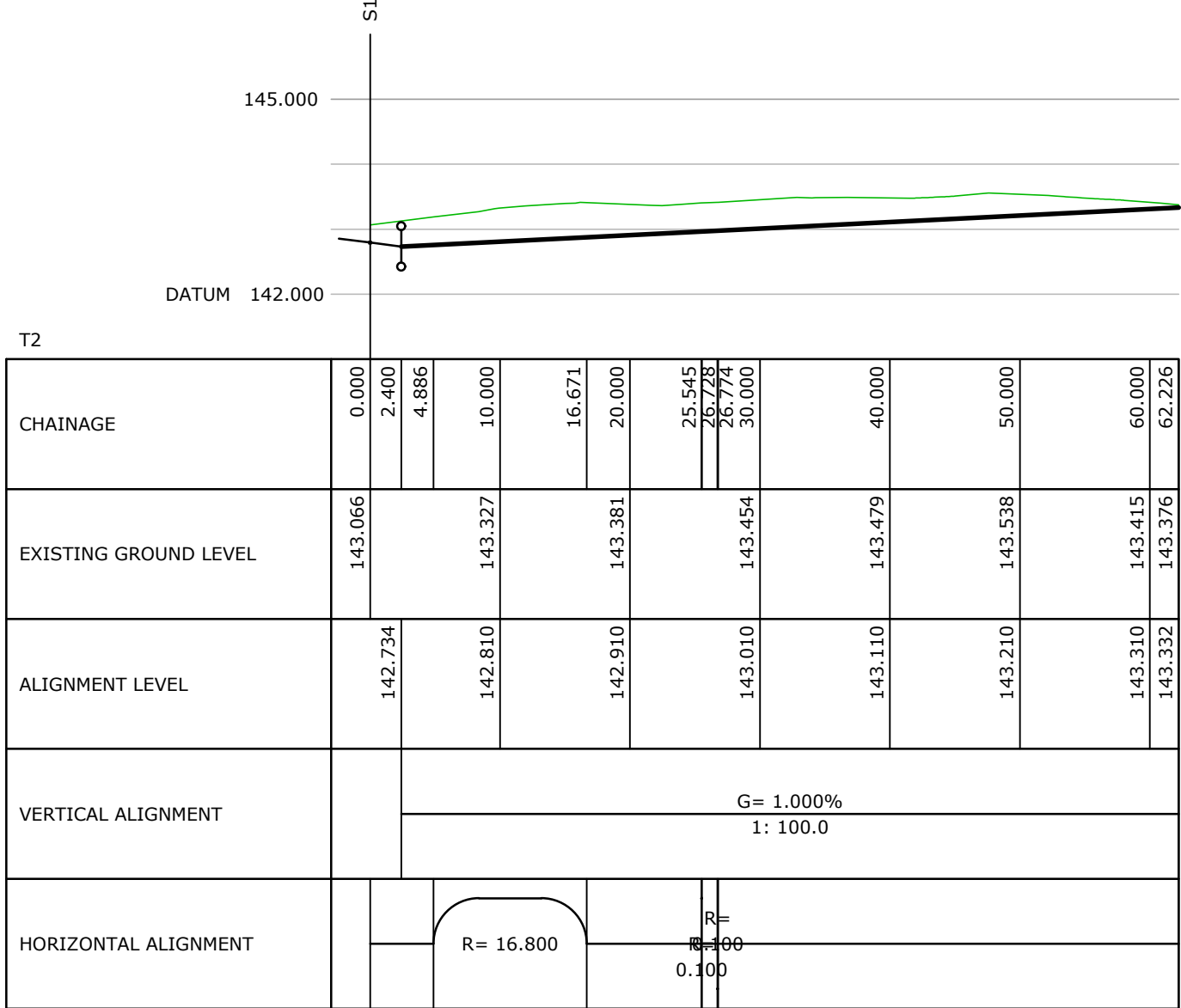
Longitudinal Section Along Tertiary Road 2
