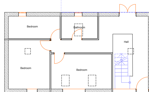
4 Existing Ground Floor Scale 1:50
