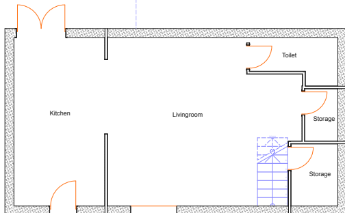
3 Existing Lower Floor Scale 1:50
