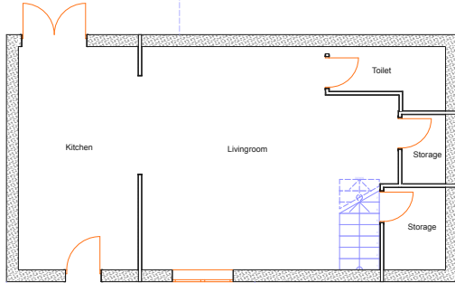
1 Proposed Lower Floor Scale 1:50
