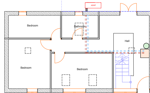
2 Proposed Ground Floor Scale 1:50
