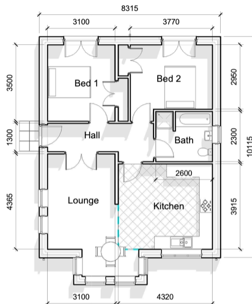
1 GROUND FLOOR 1 : 100
