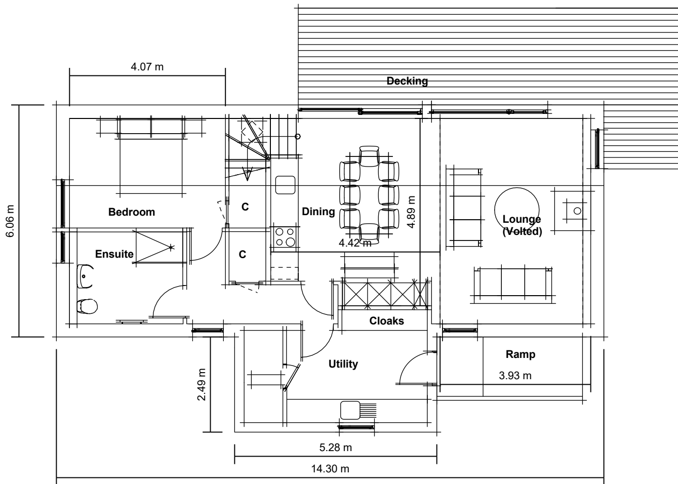
Ground Floor Plan (indicative)
