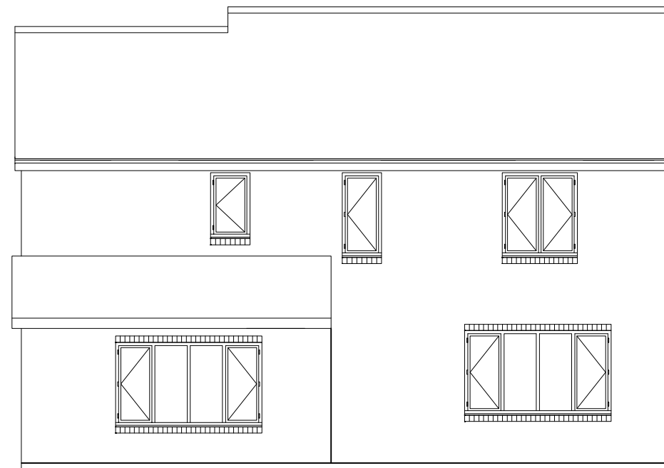
South Elevation
