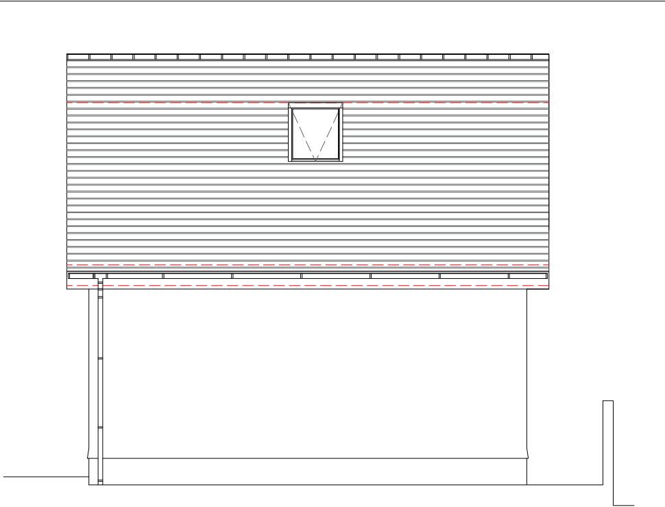
North Elevation
