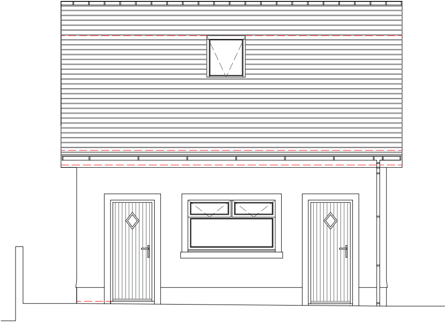
South Elevation
