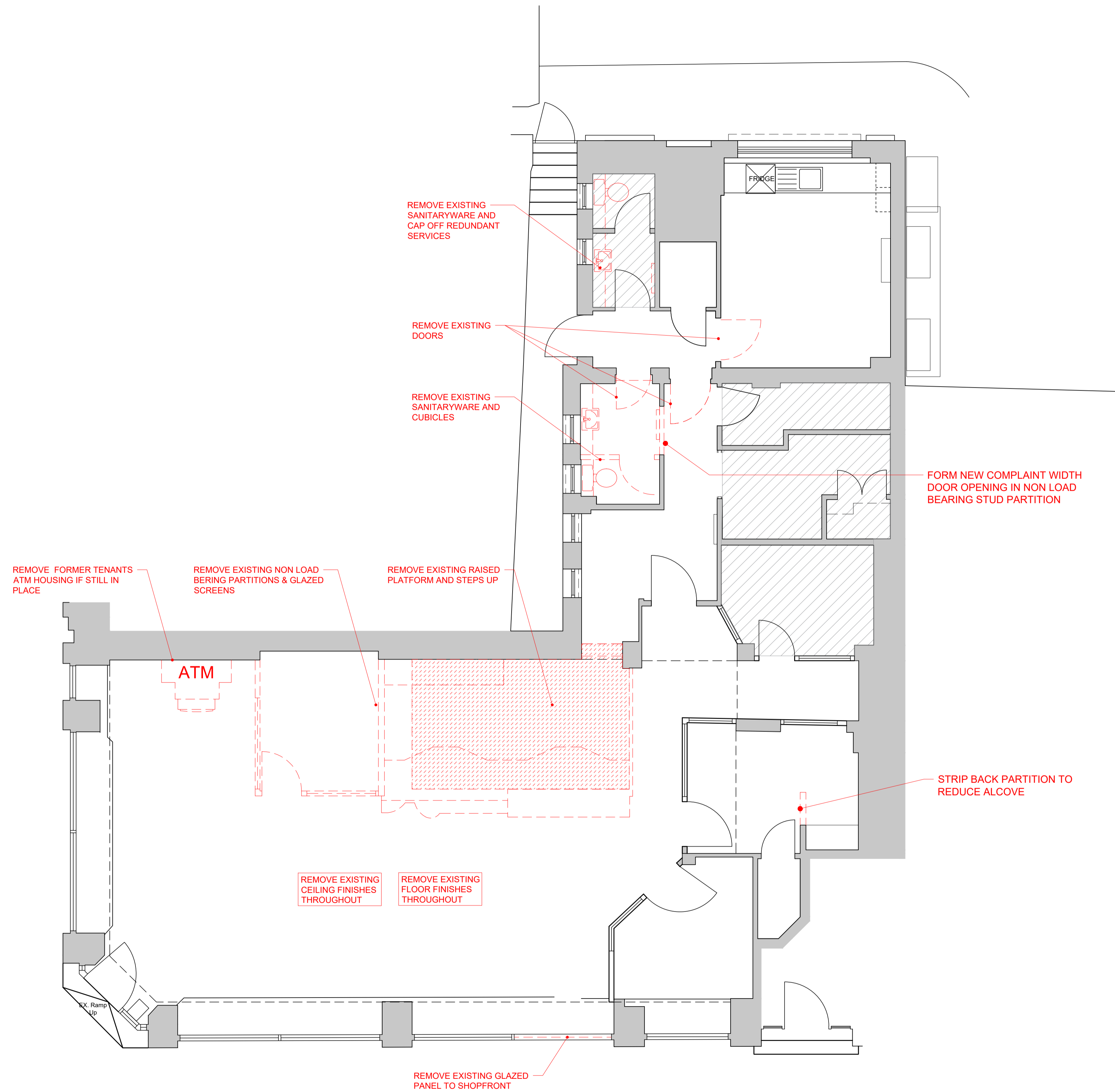
01 | Ground Floor Plan - Demolitions scale 1:50 @ A1
