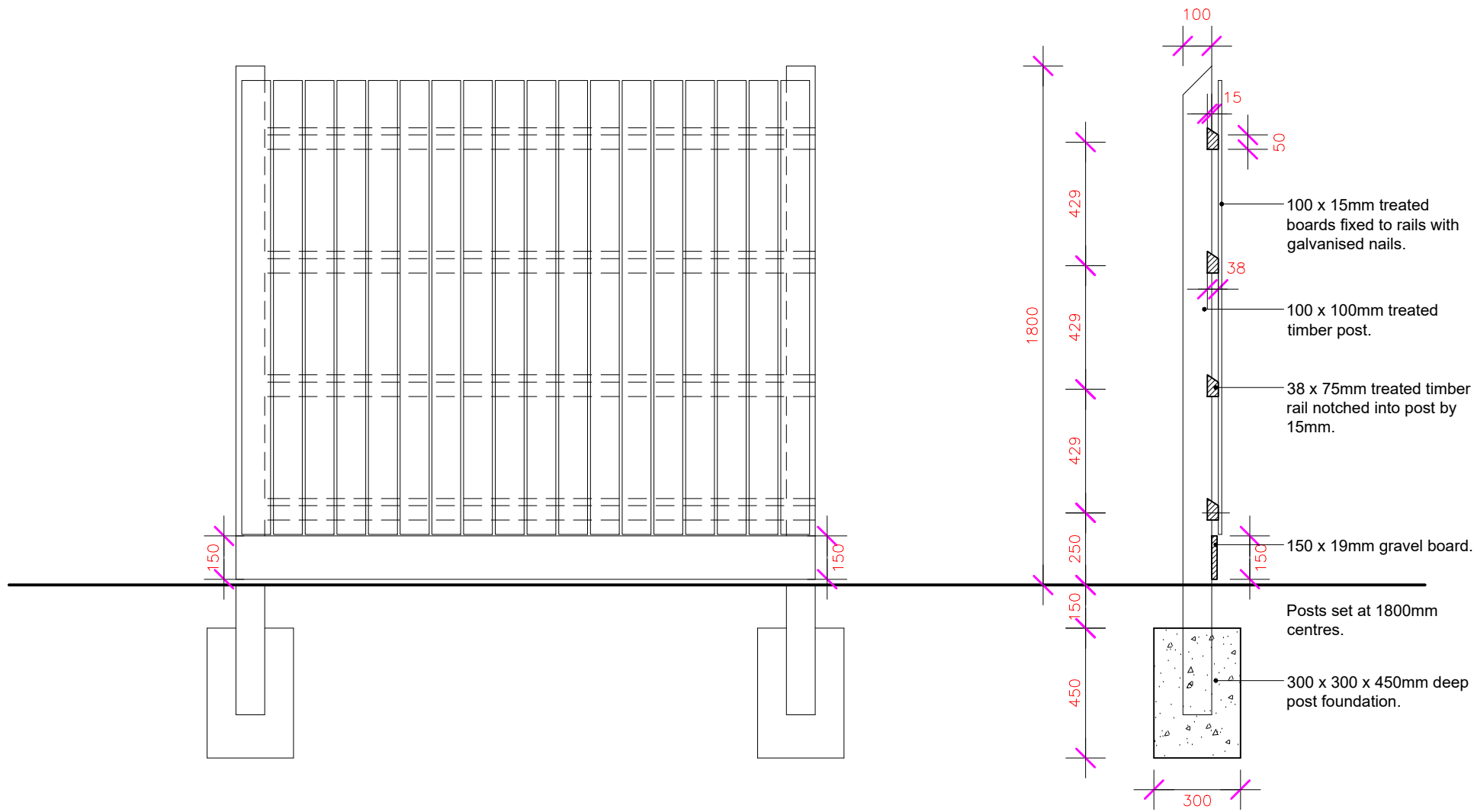
ELEVATION 1:20@A3
