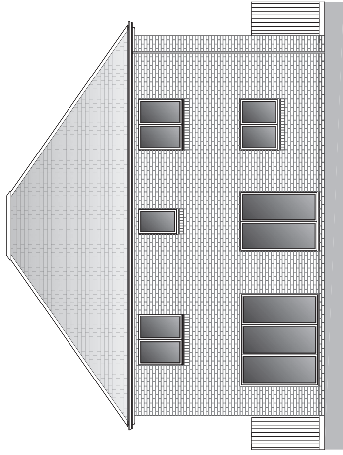
REAR ELEVATION
