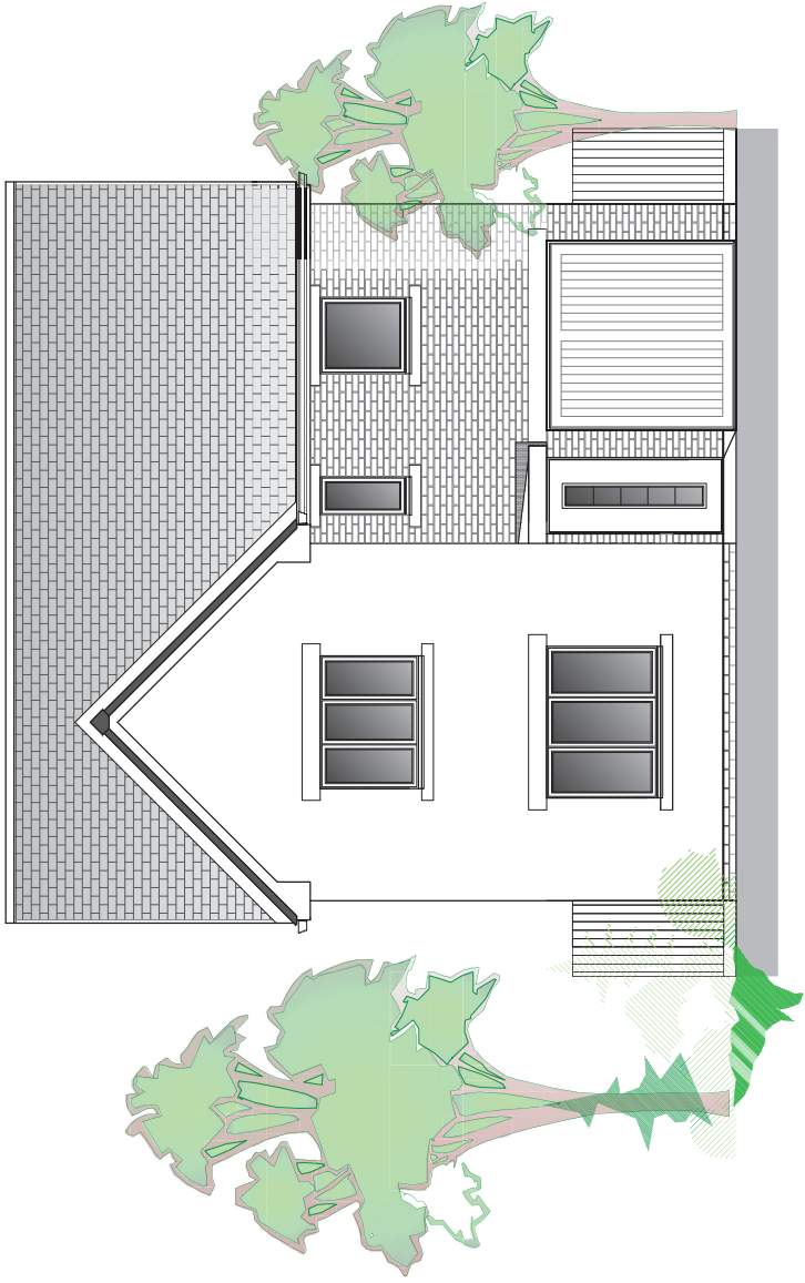
FRONT ELEVATION
