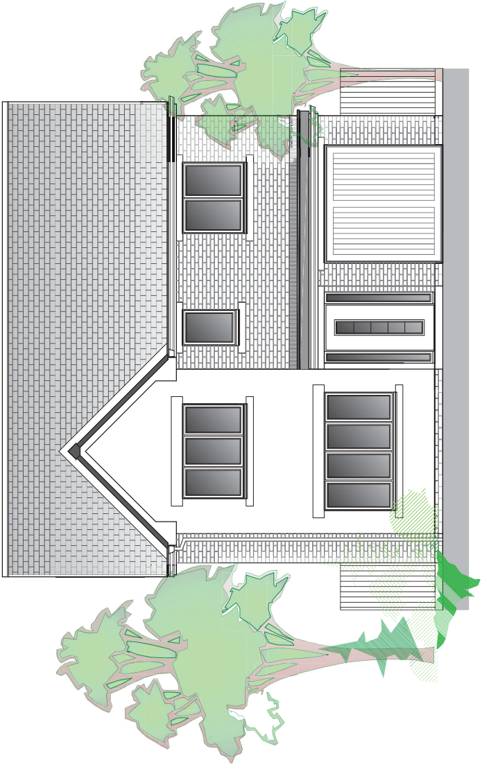
FRONT ELEVATION
