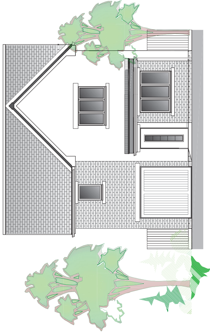
FRONT ELEVATION
