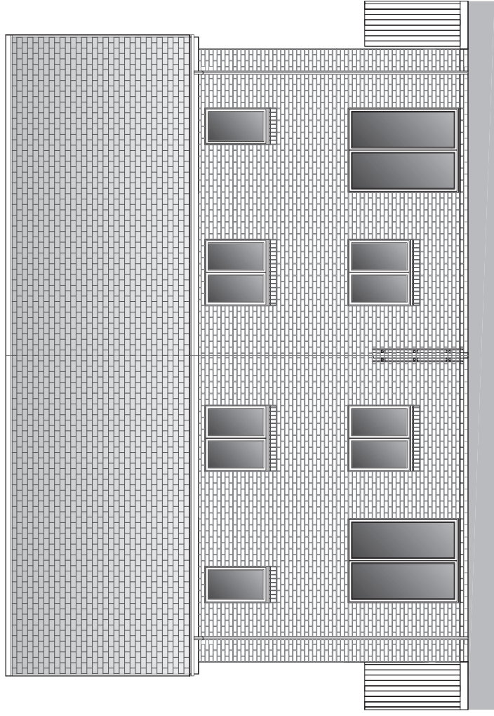
REAR ELEVATION
