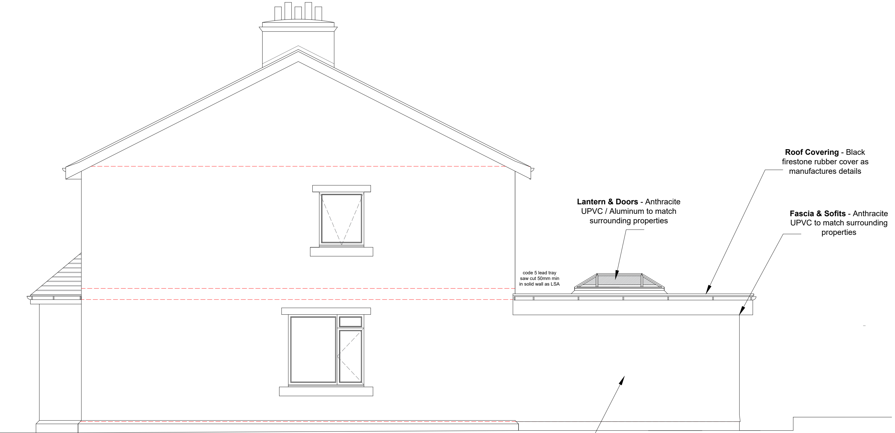
East Elevation
