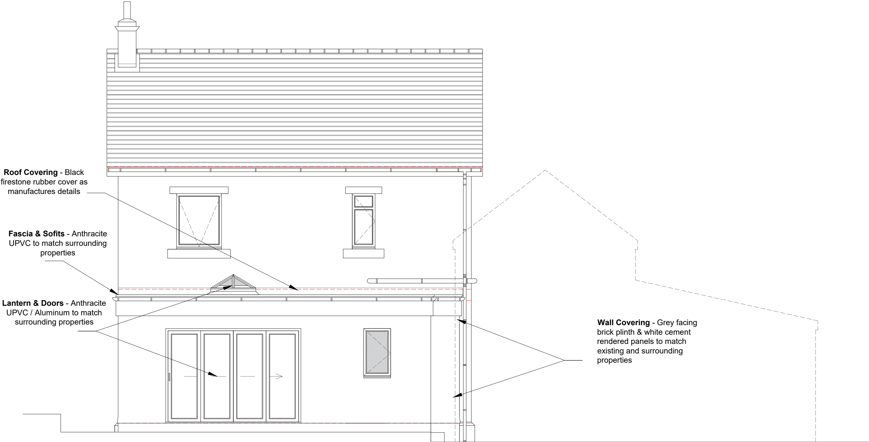
North Elevation
