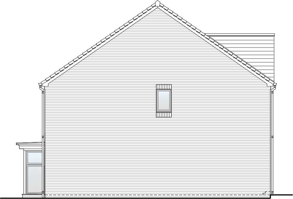
Left Elevation
