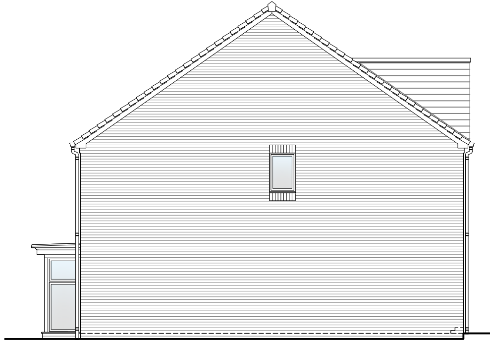
Left Elevation
