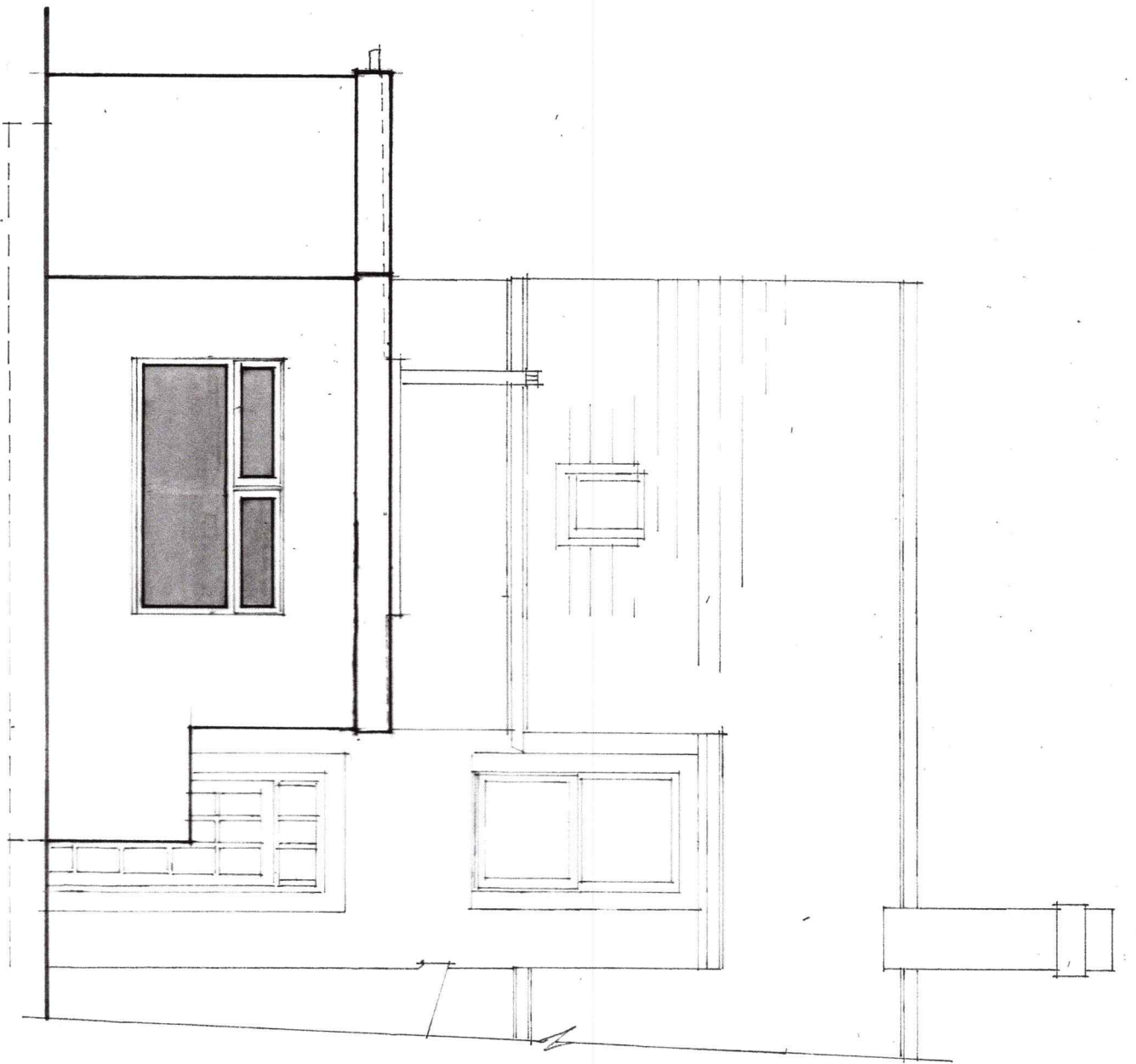
PROPOSED REAR (S)
