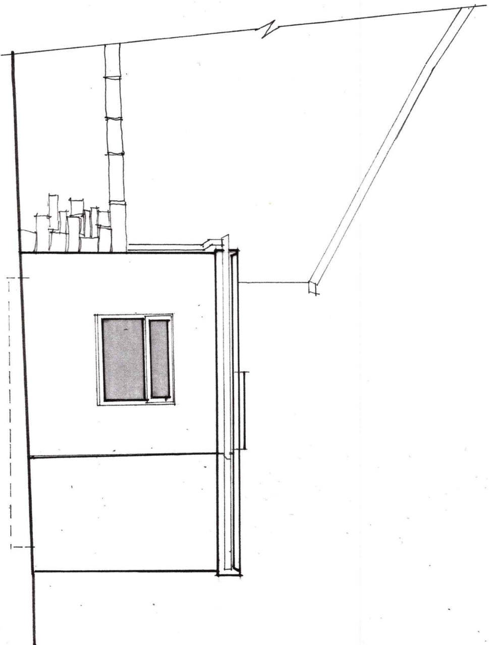
PROPOSED SIDE (W)
