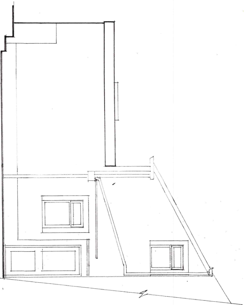
PROPOSED SIDE (E)
