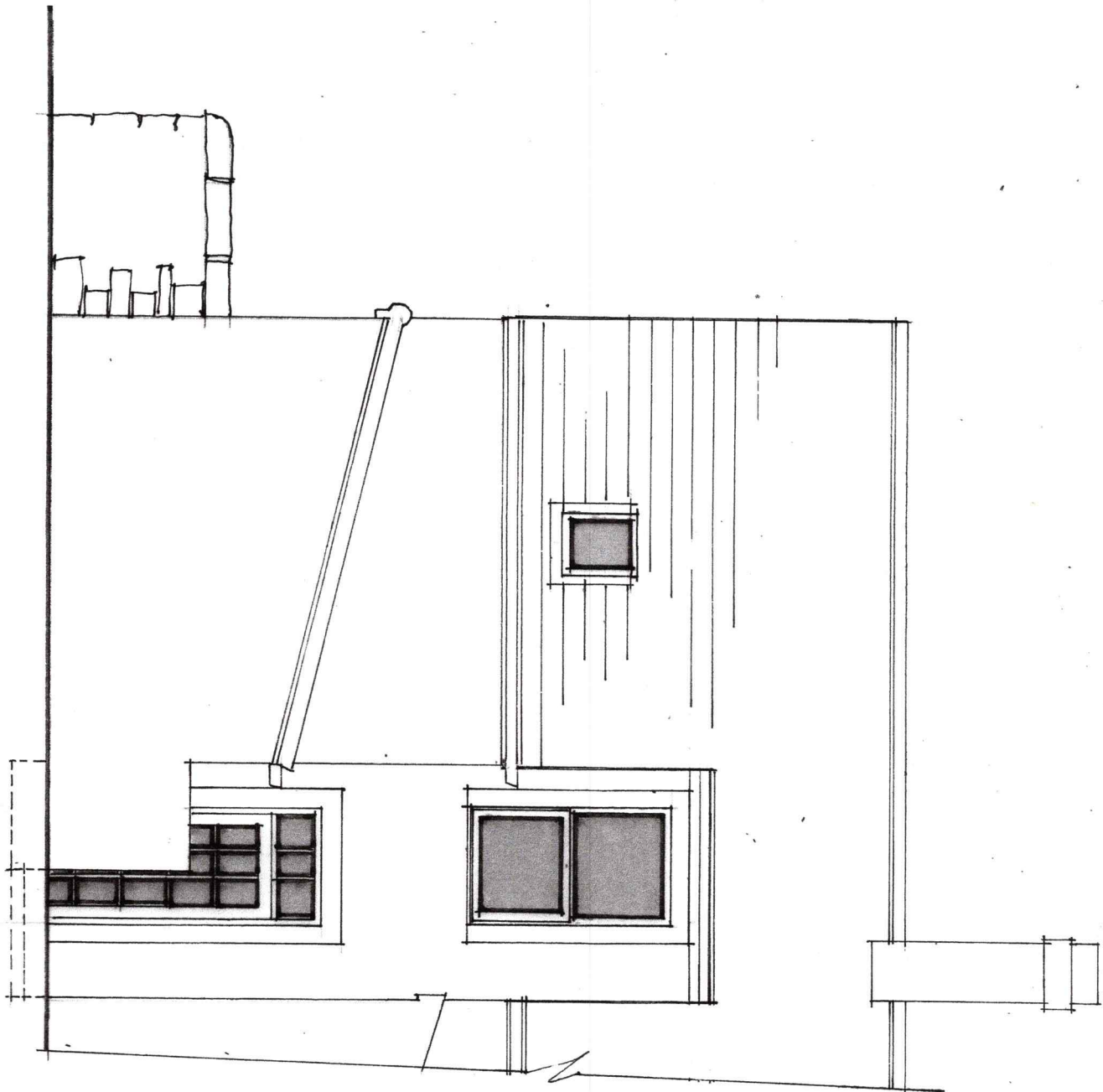
EXISTING REAR (S)
