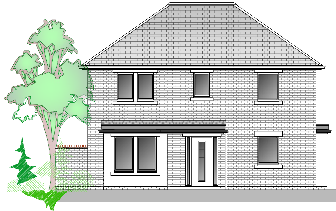
FRONT ELEVATION
