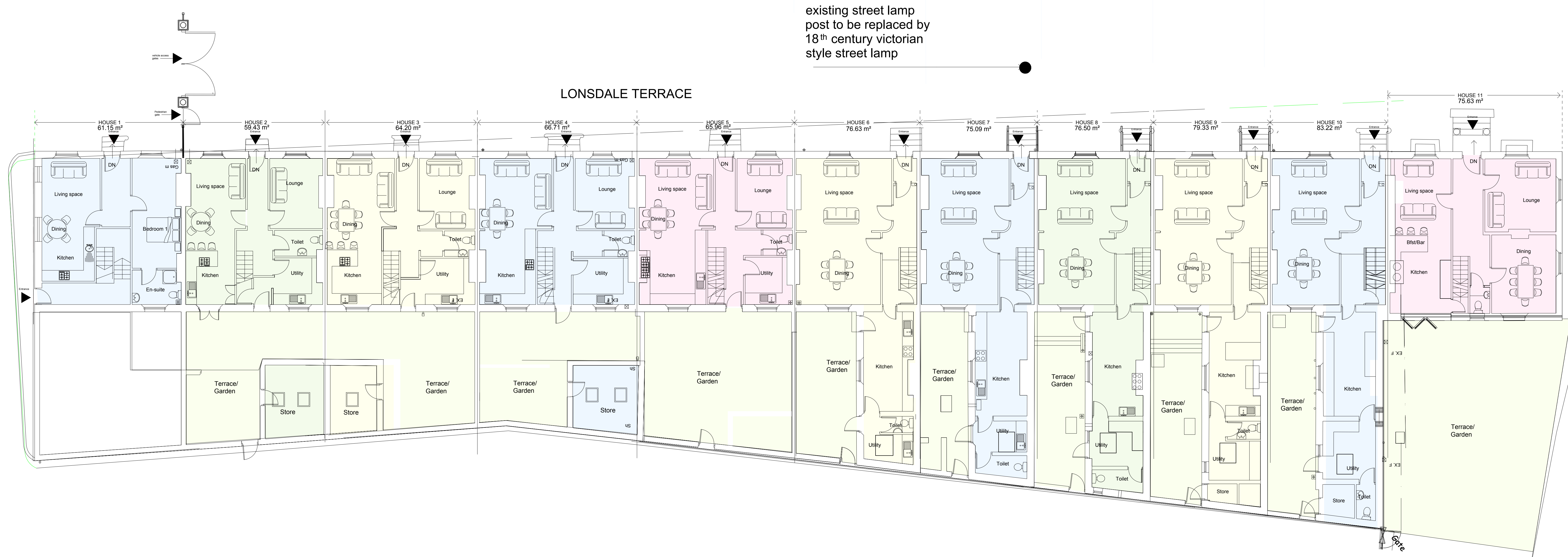
AP GROUND FLOOR PLAN 1 : 100
