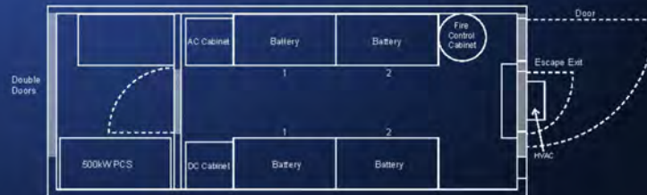
Standard 20' Container Solution 19.9x8.0x9.5 feet 100kW / 436kWh or 250kW / 763kWh
