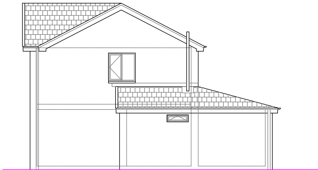
Side Elevation
