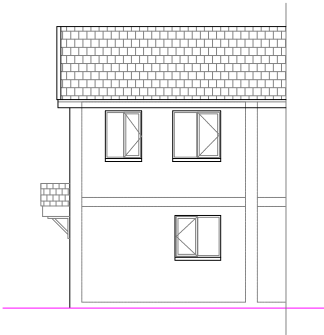
Rear Elevation
