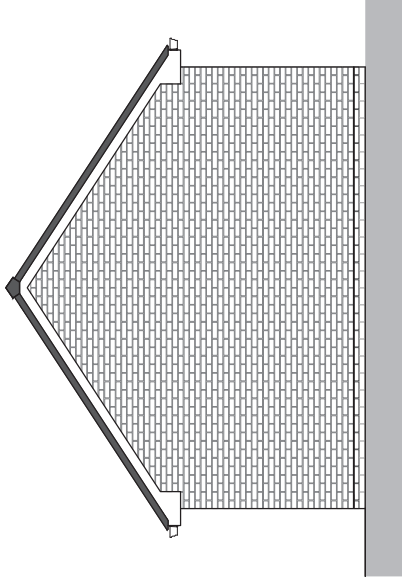
SIDE ELEVATION
