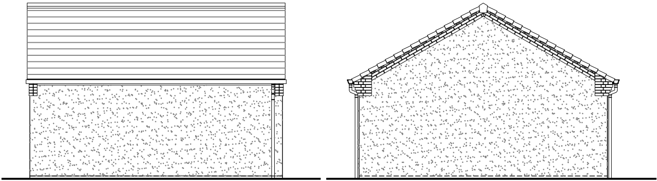
Rear Elevation
