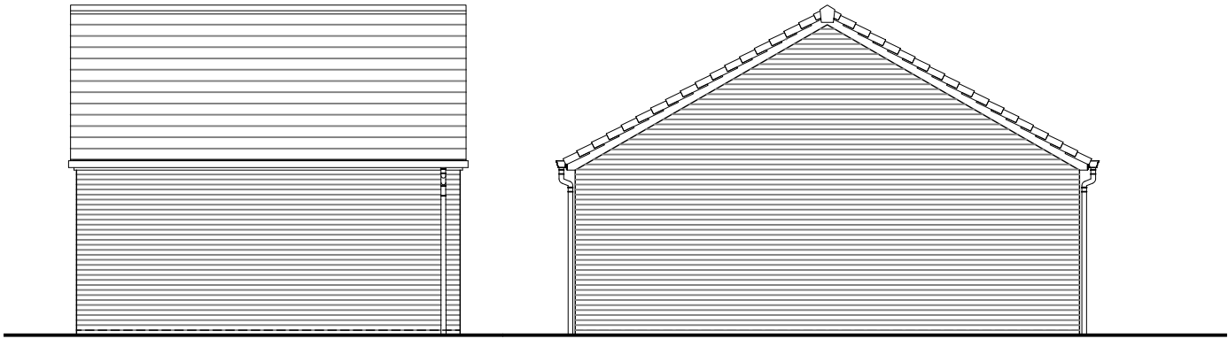
Rear Elevation
