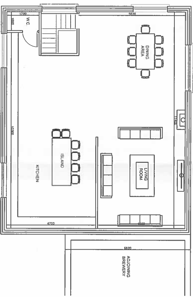
Proposed first floor plan scale 1:100 @ A3
