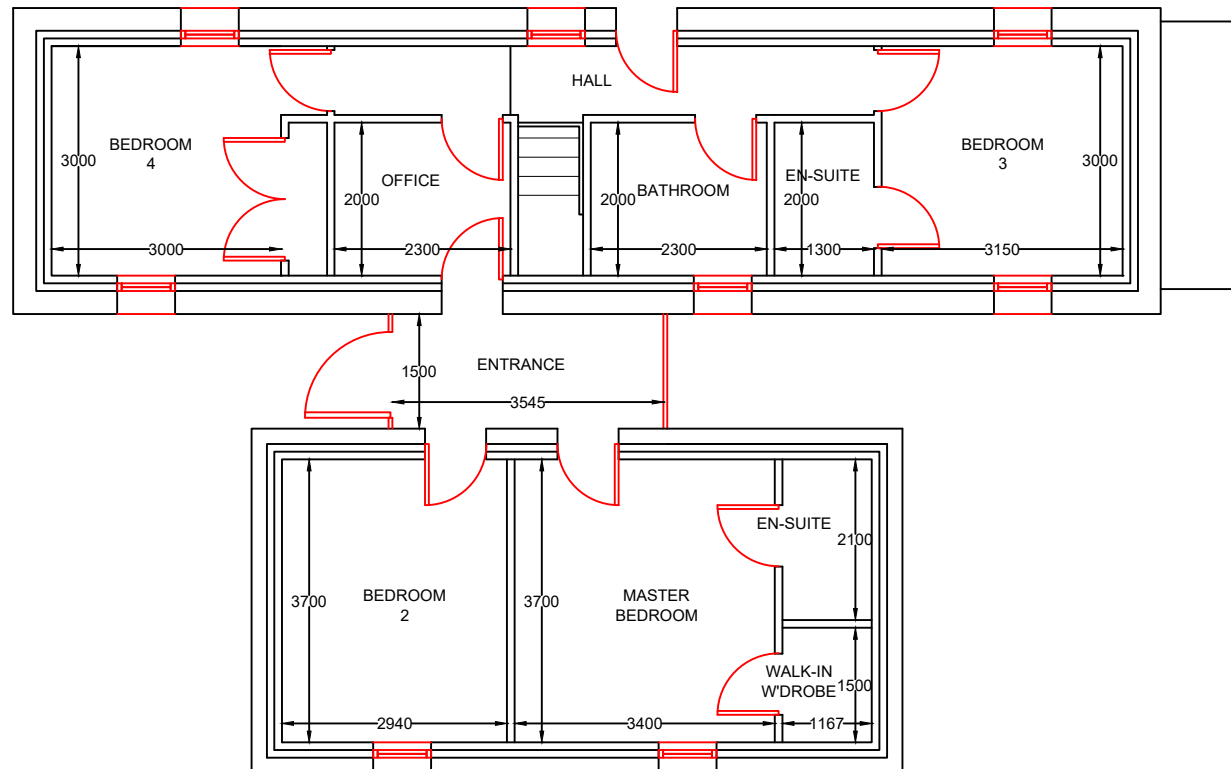
EXISTING GROUND FLOOR PLAN SCALE: 1:100 @ A3
