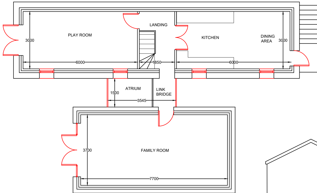
EXISTING FIRST FLOOR PLAN SCALE: 1:100 @ A3
