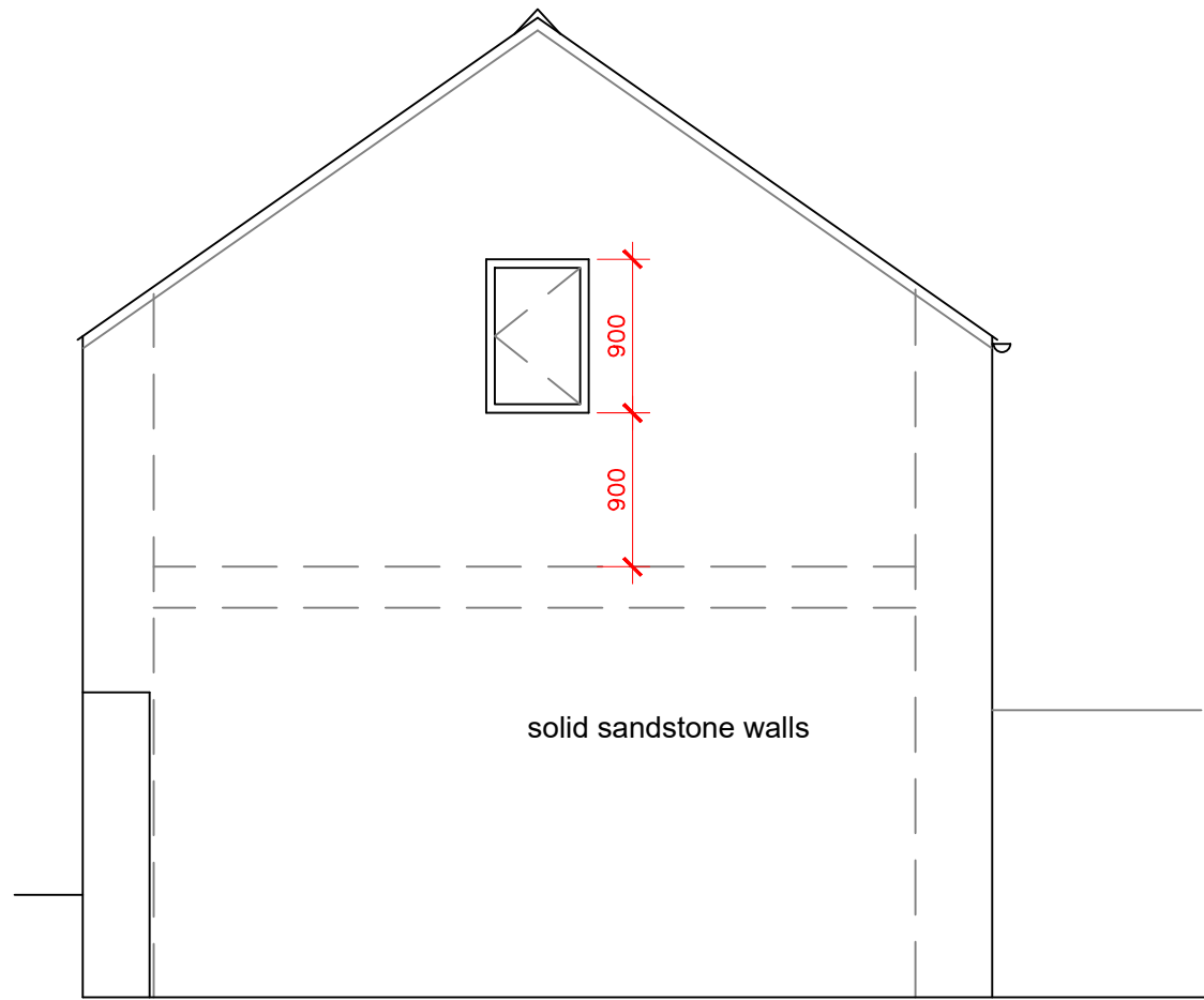
Side Elevation 1:50
