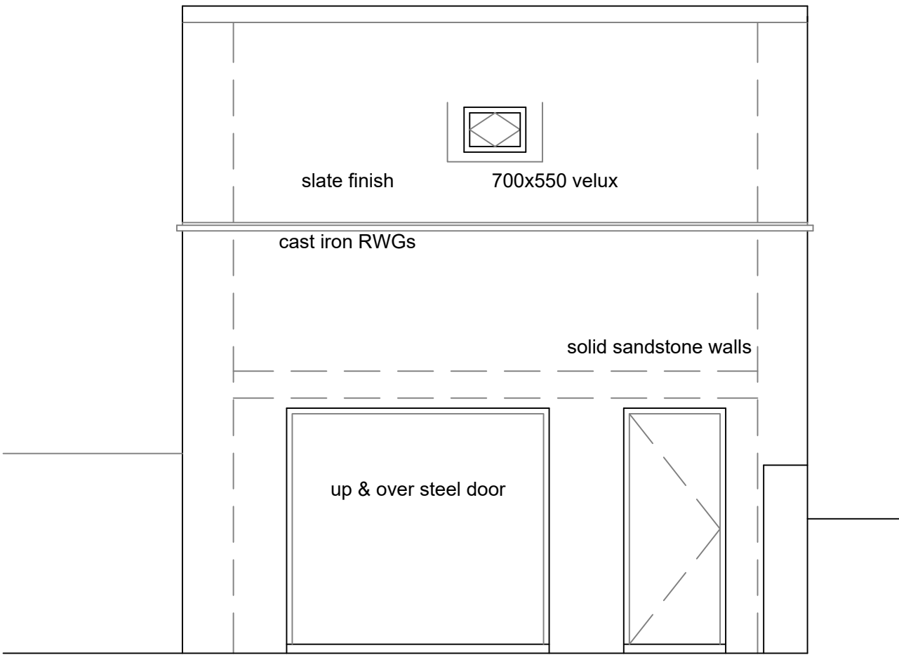
Front Elevation
