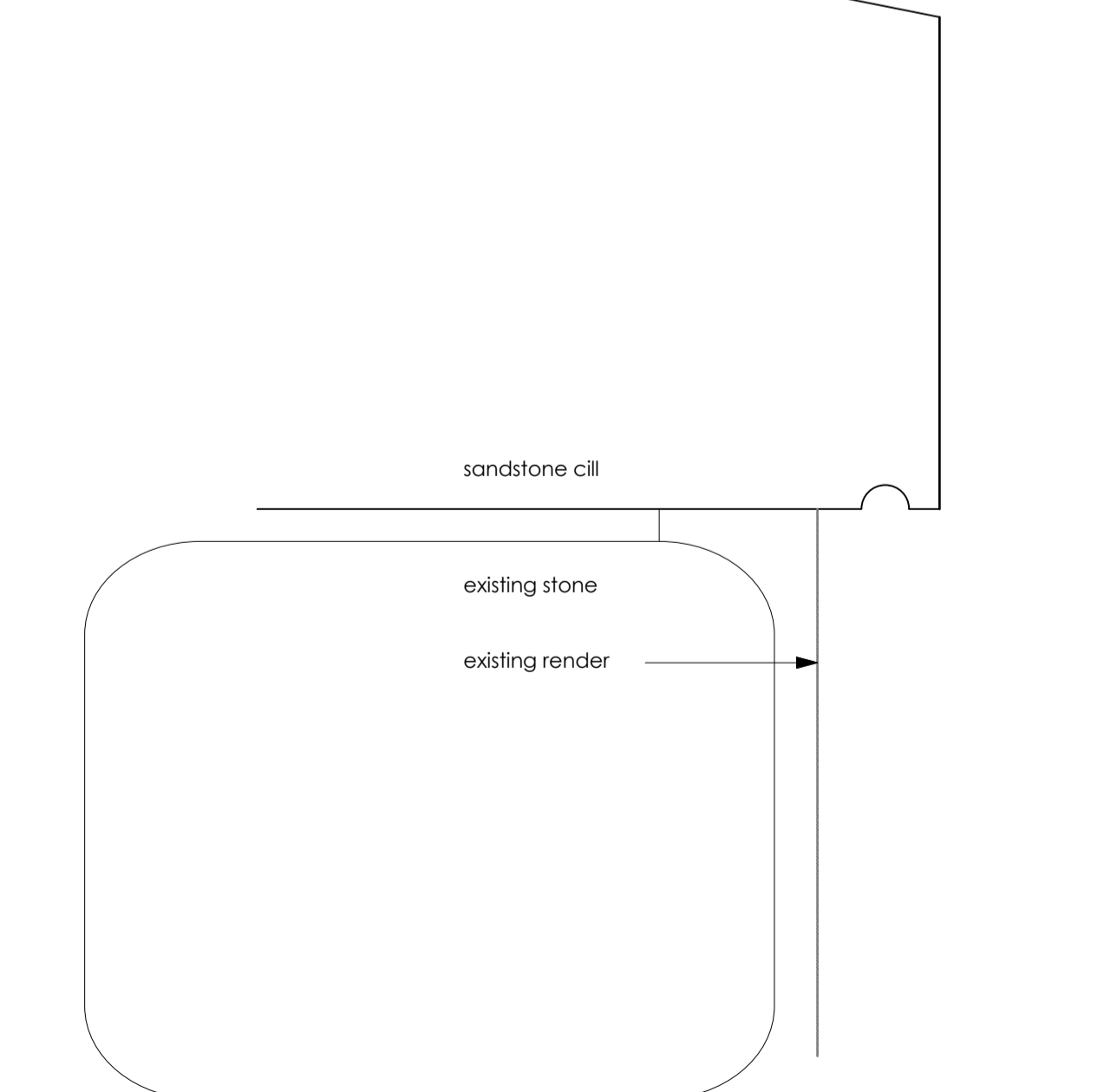
TYPICAL WINDOW SECTION NB. All timber elements are finished sizes. Timber to be hardwood (iroko) and painted REFER TO ELEVATIONS FOR NEW WINDOW LOCATIONS
