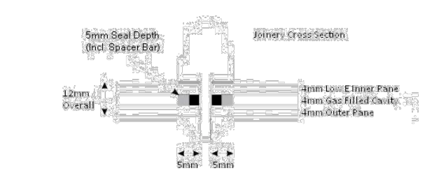
CENTRAL GLAZING BAR DETAIL
