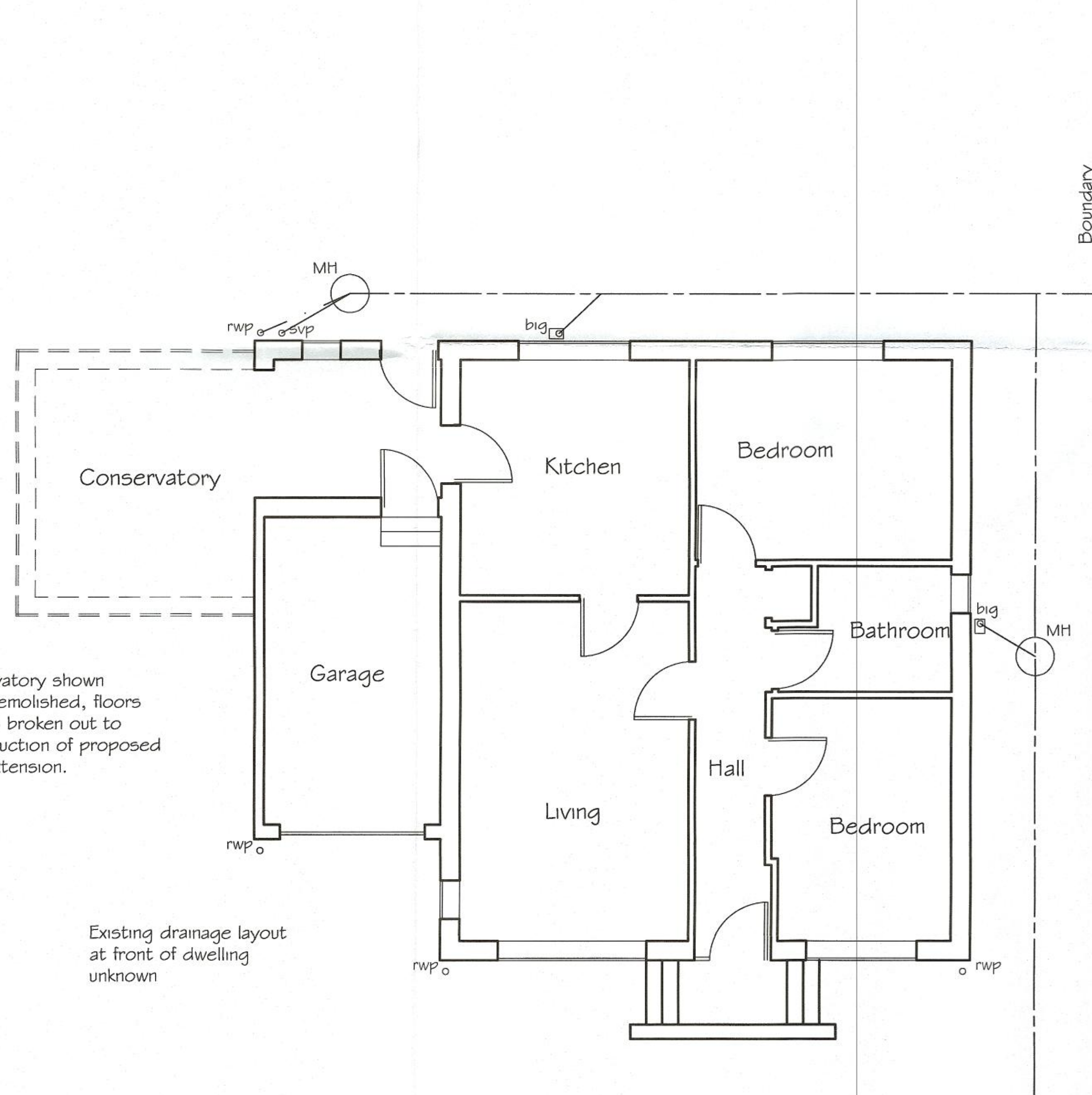
GROUND FLOOR PLAN AS EXISTING Scale 1:50
