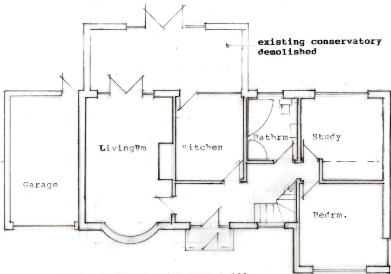
EXISTING GROUND FLOOR PLAN 1:100
