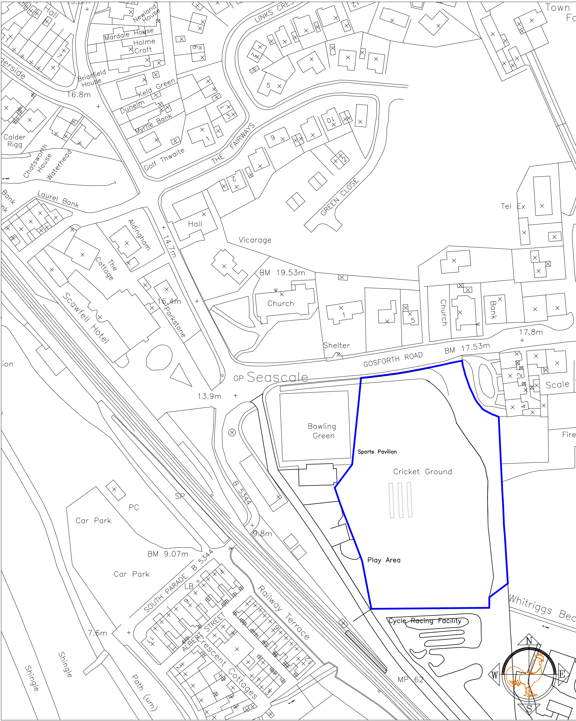
Existing Location plan Scale 1/1250
