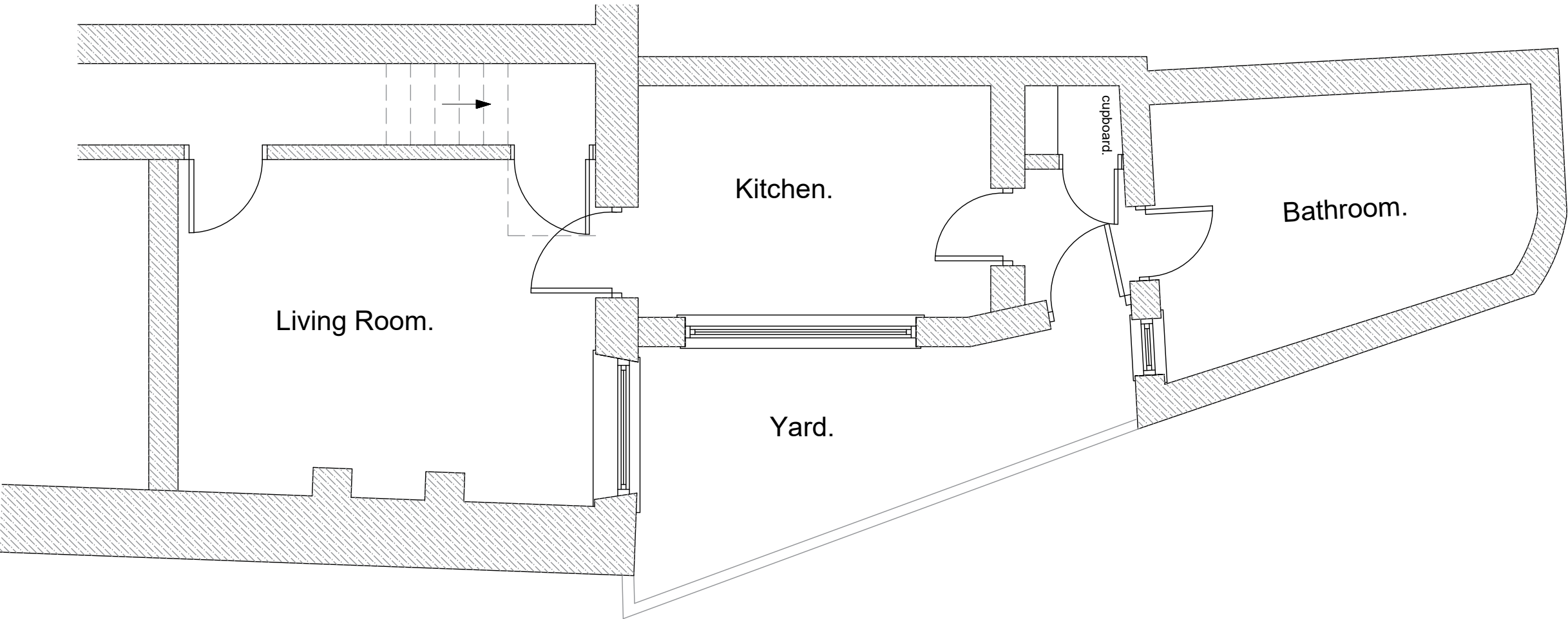
Partial Existing Ground Floor Plan
