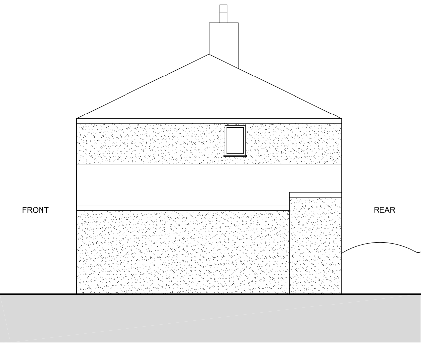
EXISTING SIDE ELEVATION (NORTH) 1:100
