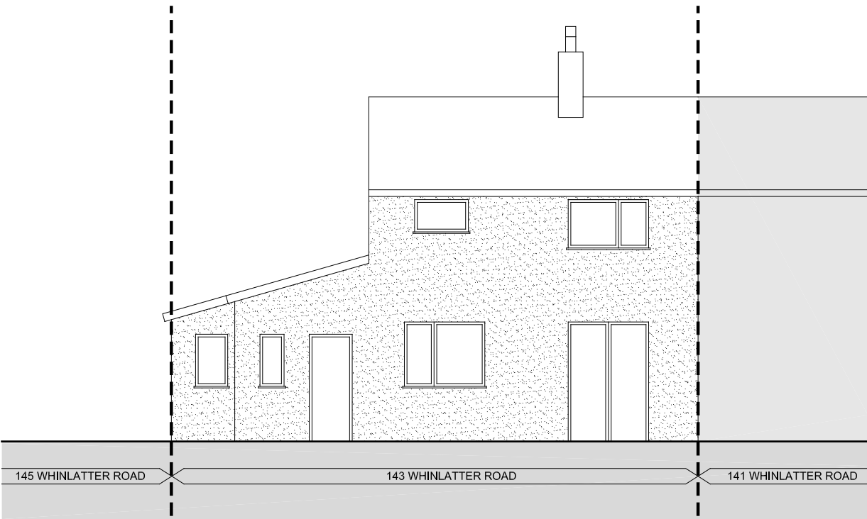
EXISTING REAR ELEVATION (WEST) 1:100
