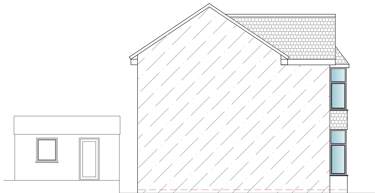
Existing Section through Adjoining Property
