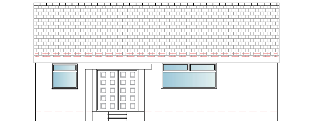
Front Elevation
