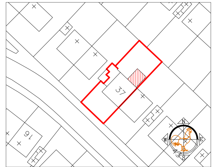
Location Plan Scale 1/500
