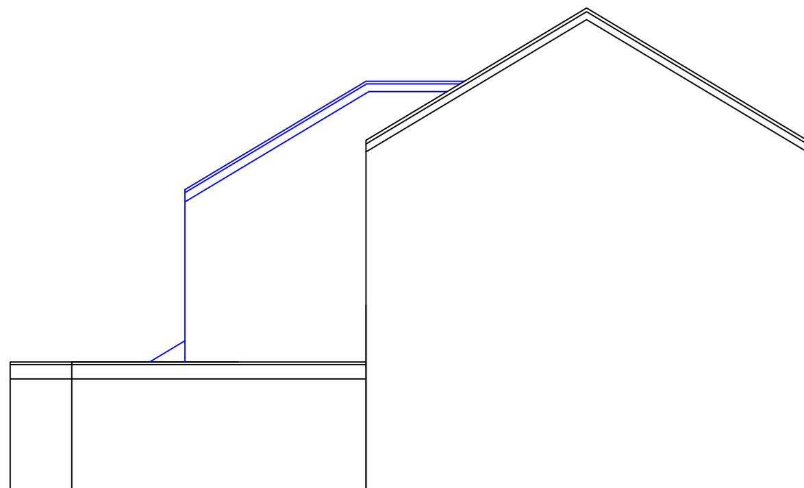
Existing Gable Elevation 2
