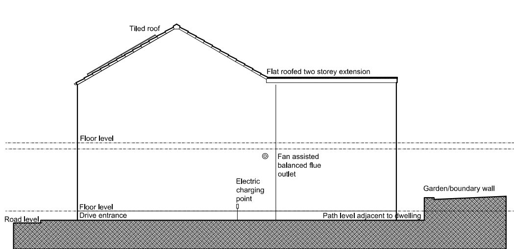
SIDE ELEVATION (SECTION THROUGH ROAD)
