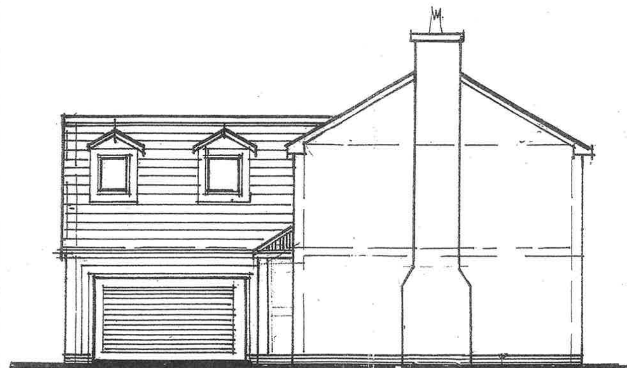
GABLE ELEVATION
