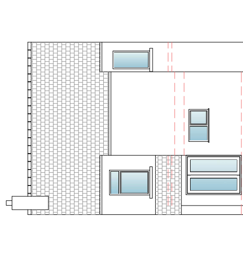
Rear Elevation
