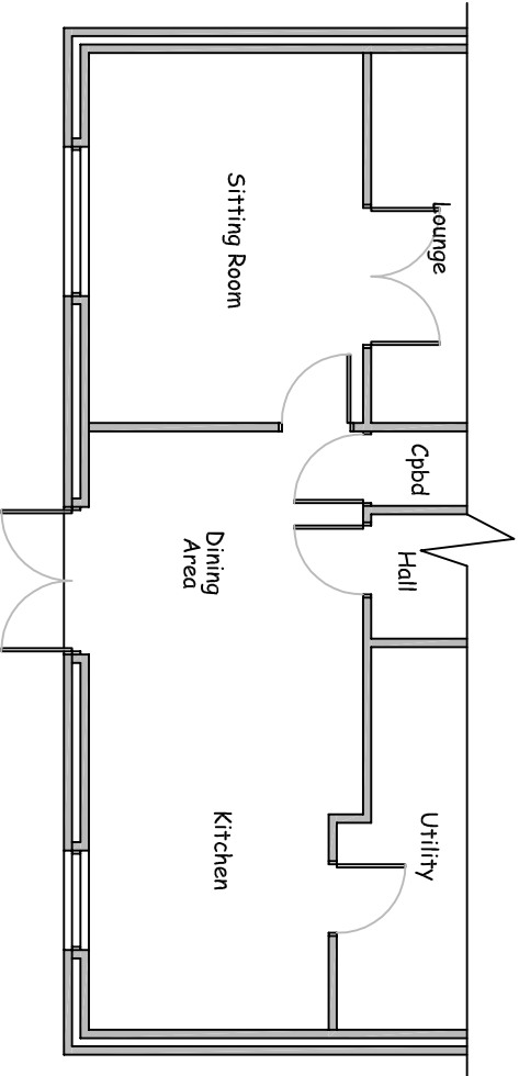
Part Floor Plan
