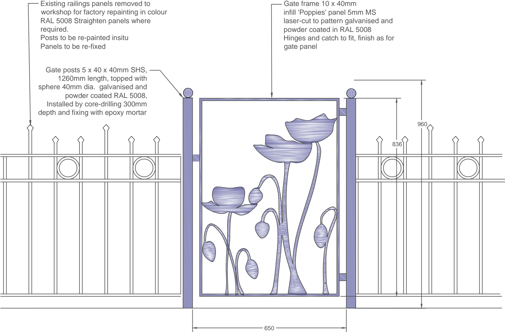
NEW GATE TO WAR MEMORIAL AND REFURBISHED RAILINGS 1:10
