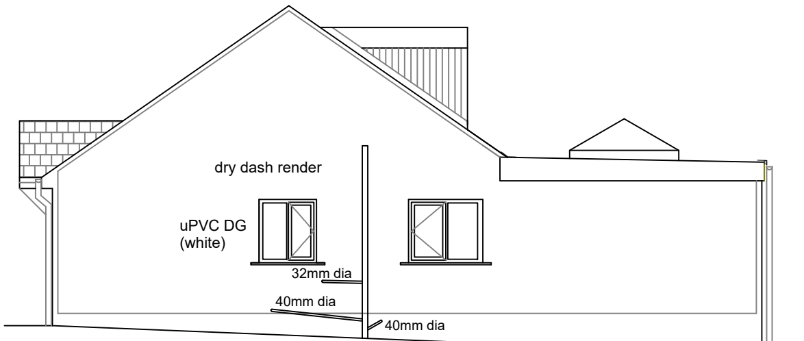
Side Elevation
