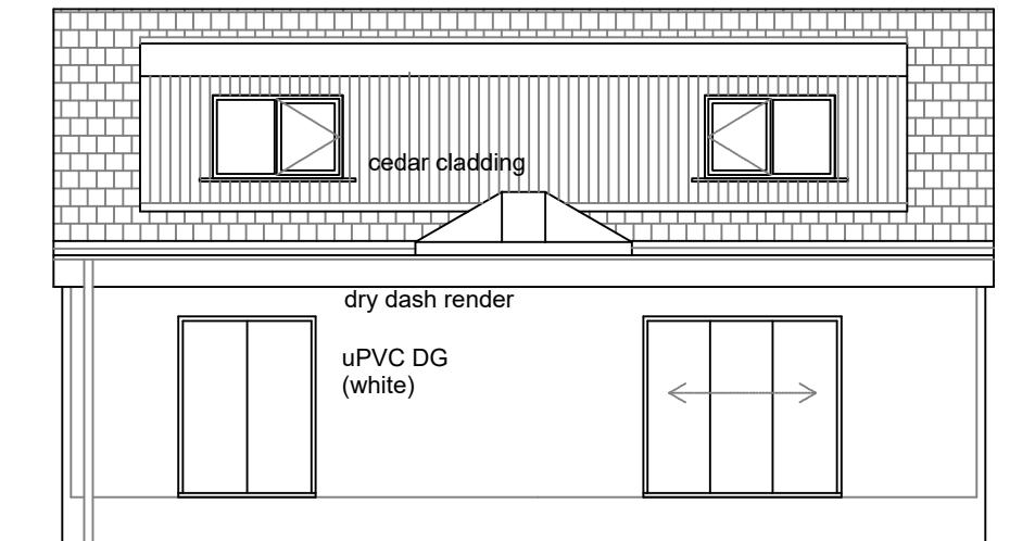
Rear Elevation
