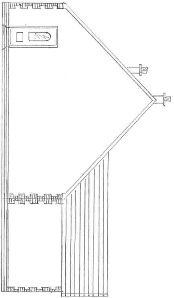
EXISTING EAST ELEVATION < 1:100 >
