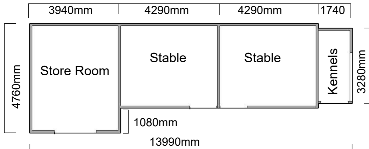
Floor Plan
