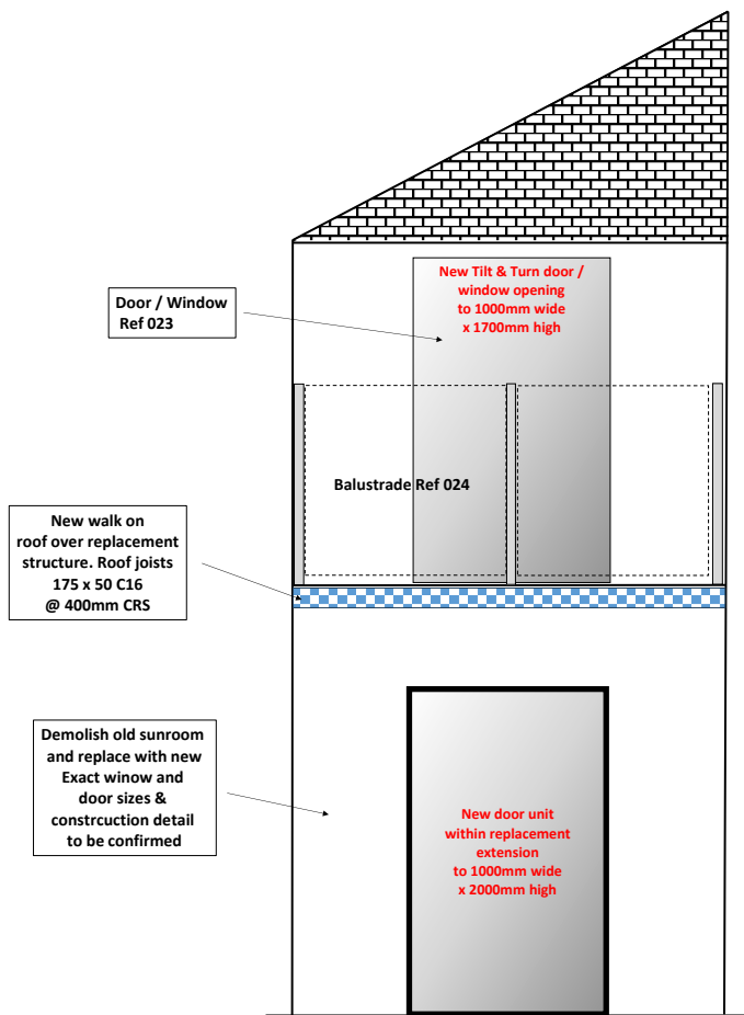
West Elevation - Proposed Door Detail on to New Balcony
