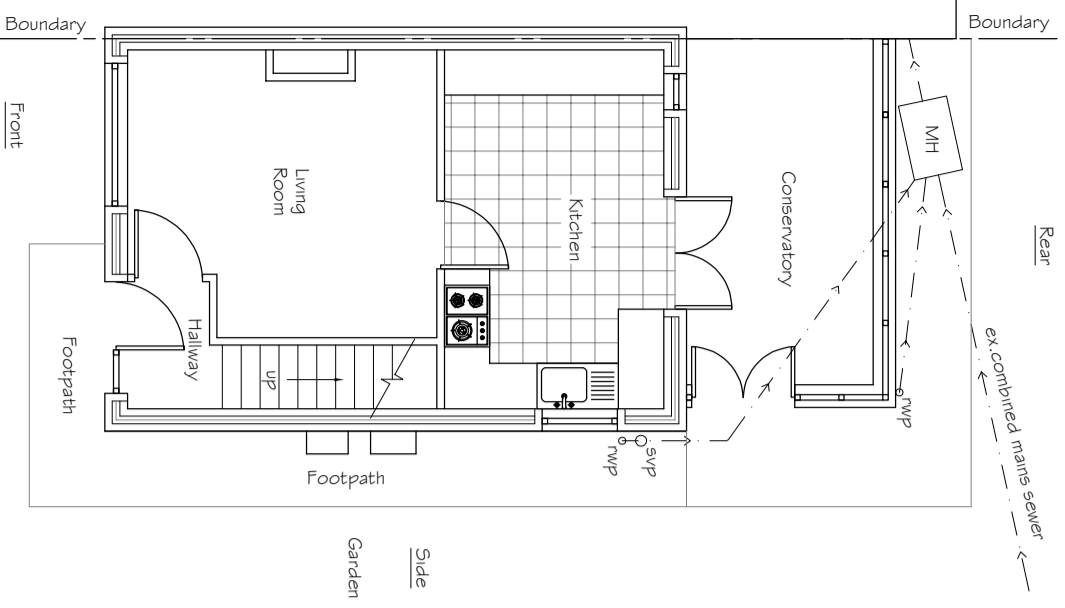
GROUND FLOOR PLAN AS EXISTING Scale 1:50
