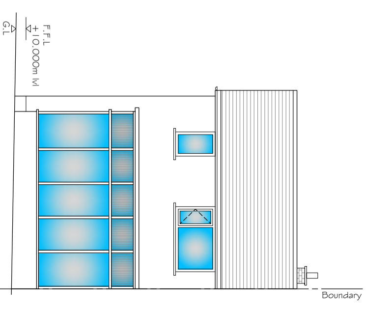
REAR ELEVATION AS EXISTING Scale 1:50
