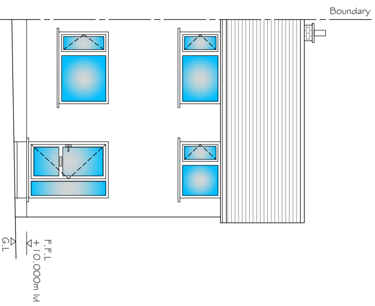
FRONT ELEVATION AS EXISTING Scale 1:50
