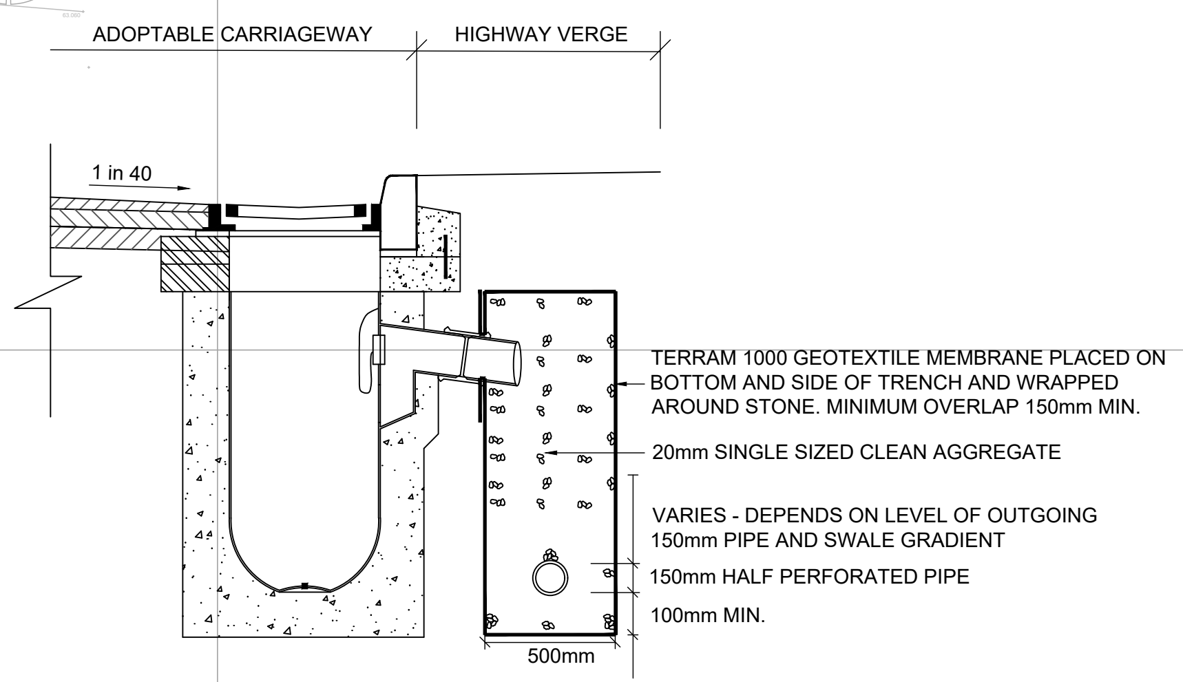
SECTION THROUGH HIGHWAY DRAINAGE FILTER DRAIN (HIGHWAY VERGE) (SUBJECT TO THE APPROVAL OF THE HIGHWAY AUTHORITY)
