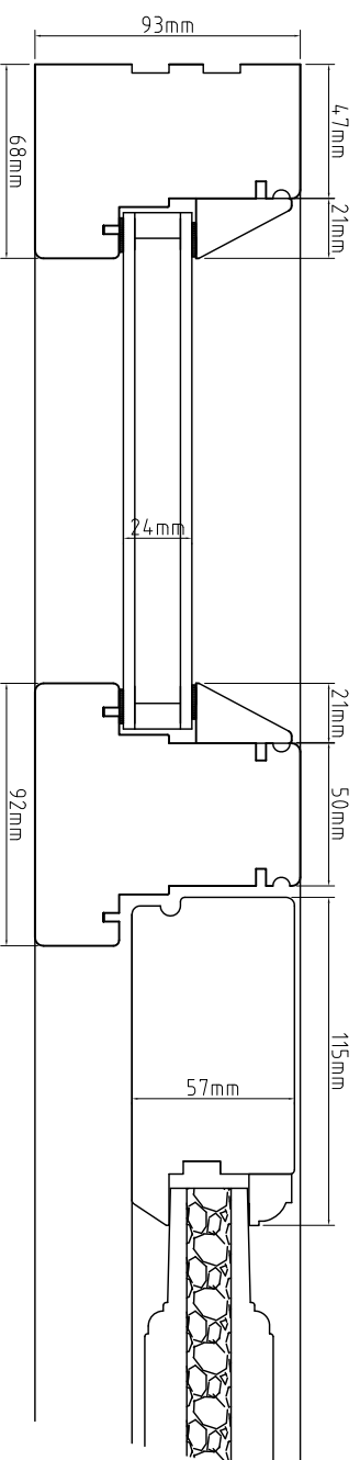
SECTION THROUGH MULLION A-A
