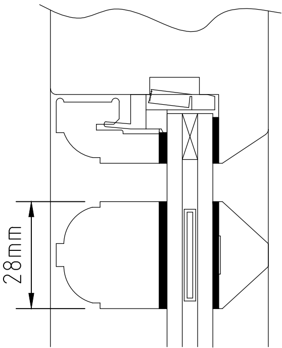
12mm GLAZING
