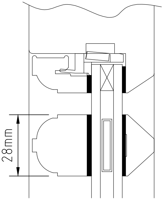
14mm GLAZING
