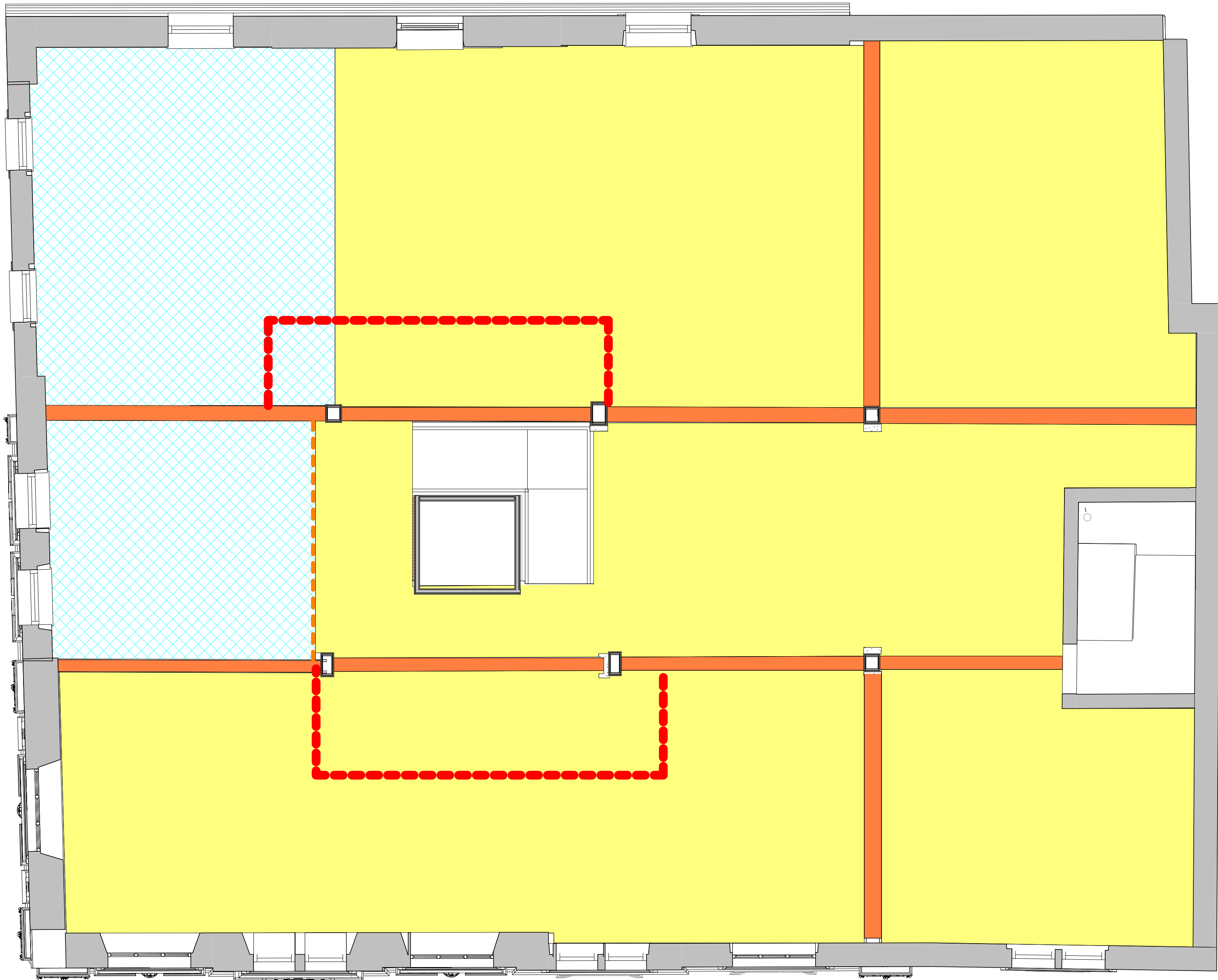
LEVEL 01 CEILING LININGS SCALE: 1 : 50
